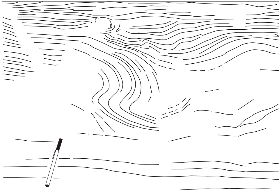
Photo 2. Location 1-a, base of cliff, Rockcliffe Parkway (see Photo 1). 15 cm pen for scale. Folded laminations within a horizontal, fine-grained sandstone bed of the Rockcliffe Formation. The folds reflect 'soft-sediment' deformation within the bed when the sand was saturated with water and unconsolidated.
