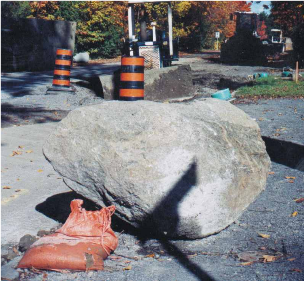
Photo 16. Location 5-a, Birch Avenue at corner with Hemlock Road. Erratic boulder dug from marine clay (unit 5) beneath Birch Avenue, October 2003. Boulder is composed of layered crystalline gneiss, a rock metamorphosed (changed) under conditions of high temperature and pressure. Similar rock is associated with granites in the Gatineau Hills.
