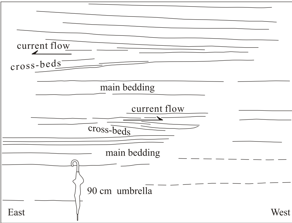
Photo 1. Location 1-a, cliff face, Rockcliffe Parkway. Cross-beds in fine-grained sandstones and shales of the Rockcliffe Formation. Opposite inclinations of cross-beds at different levels indicate changes in direction of current flow.
